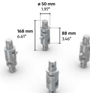
MRT1-07B|Hinges|4pcs
