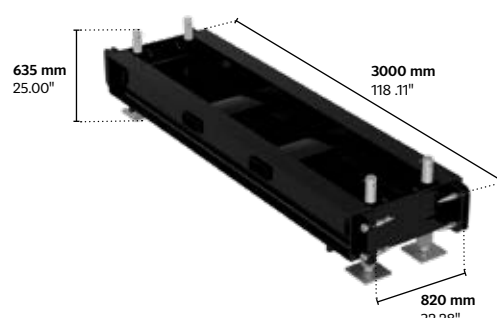
S-MT-Q-05|Outrigger3000
