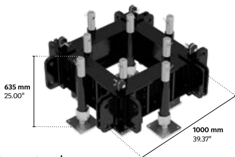
S-MT-Q-01|Base
