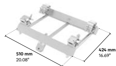
MRT1-05|StabilizerVertical
