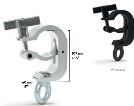
CELL603 / CELL603|Anodised
