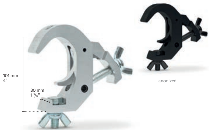
CELL402 / CELL402|anodized Quick clamp with bolt and wingnut
