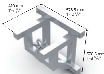
MT2-09|BracketForMotor|Sleeve
