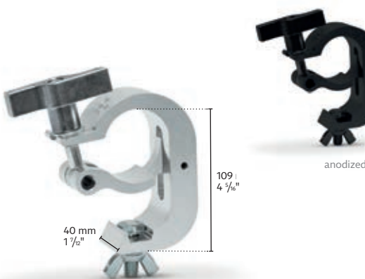
CELL602 / CELL602|anodized Basic clamp with bolt and wingnut
