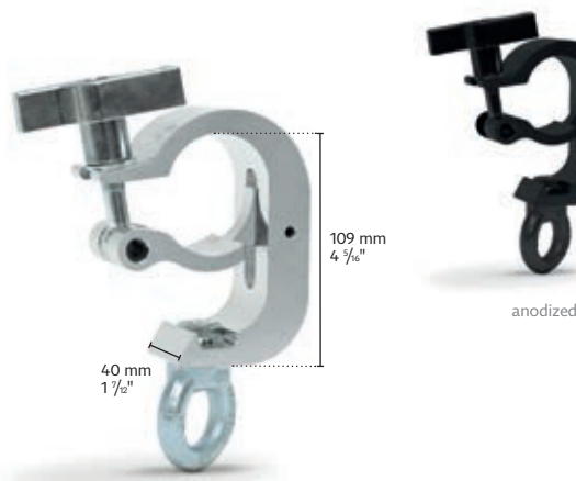
CELL603 / CELL603|anodized Clamp with lifting eye
