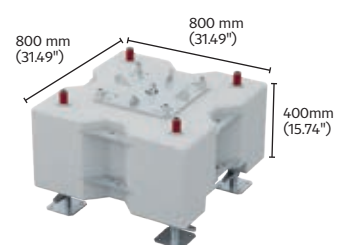
Concrete Ballast Base MCBB
