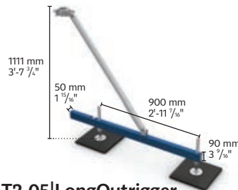
MT2-05|LongOutrigger
