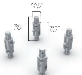
MRT1-07B|Hinges|4pcs
