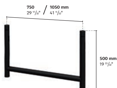
MLA-H750x500|color MLA-H1050x500|color
